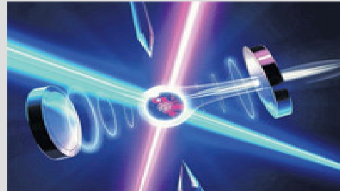
Quantum Optics
