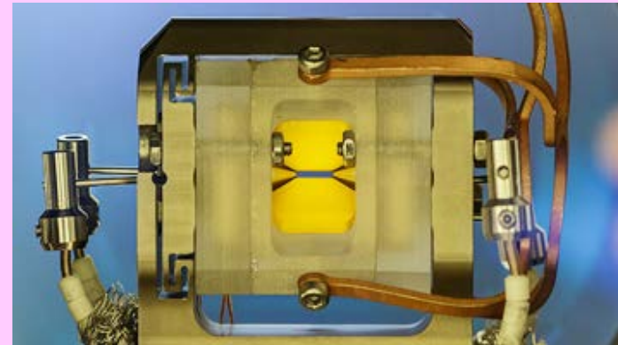
Ion-traps
